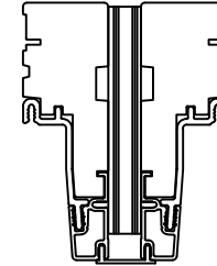
1/2" X 3 1/2" LVL MULL PROFILE
