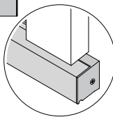
Sill nose and 3 1/2" (89) flat casing with 1" (25) extended corner
