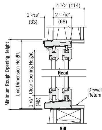
Vertical Section
